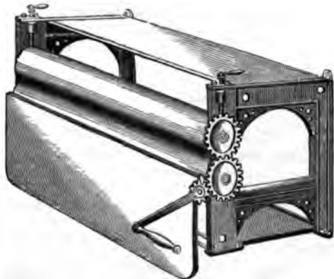
Stutterd's New Elastic Pressure Mangle.
