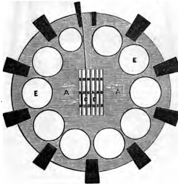
Ground Plan.—A, "Siege" or Floor of Furnace. BB, Pillars, which support the Crown. CC, Grates. D, Furnace Door. EE, Position of Crucibles.
