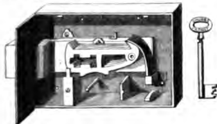
Chubb's Patent Detector Lock and Key.
