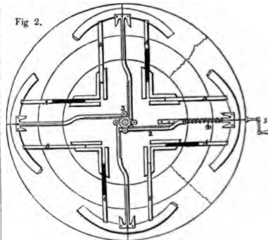
Hawkins's Patent Cog-wheel Movement for Dining-tables.
