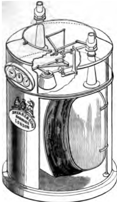
Shears & Son's Patent Dry Gas-meter.
